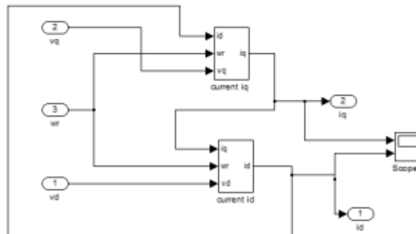
Fig.5. id,iq current blocks
