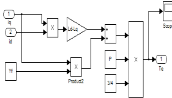
Fig.7. Torque model blocks of PMSM
