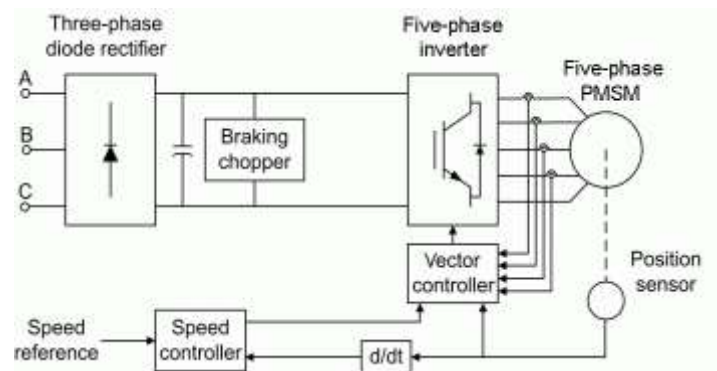
Fig 10. Proposed five phase PMSM modeled block diagram
