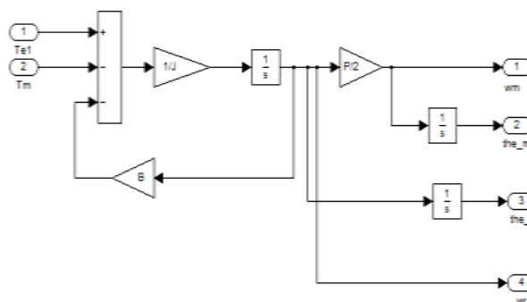
Fig.6. Speed model blocks
